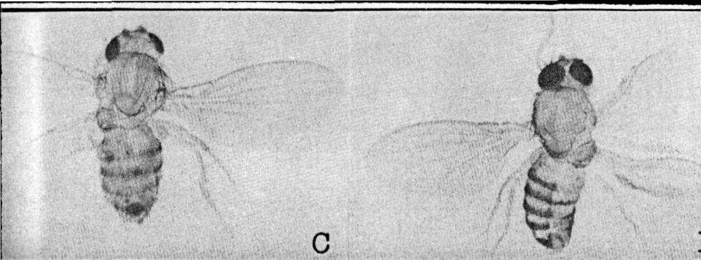
ing gene mutation through X-irradiation and chromosome rearrangements. A is a normal male Drosophila; B is a four-winged male with a double thorax; and C and D are three-winged flies with partial double thoraxes.
